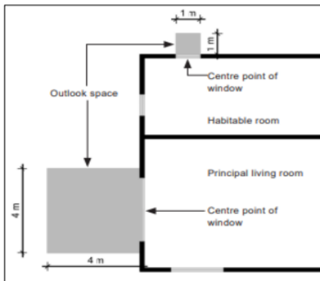
Figure I339.6.1.7.1 Outlook space requirements
