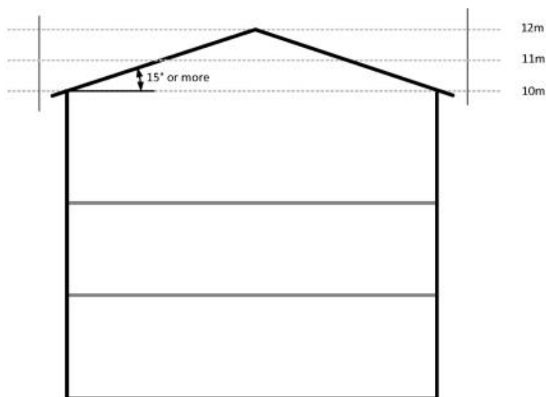
Figure I339.6.1.2.1 Building height
