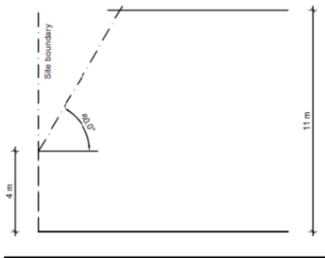
Figure I339.6.1.3.1 Height in relation to boundary
