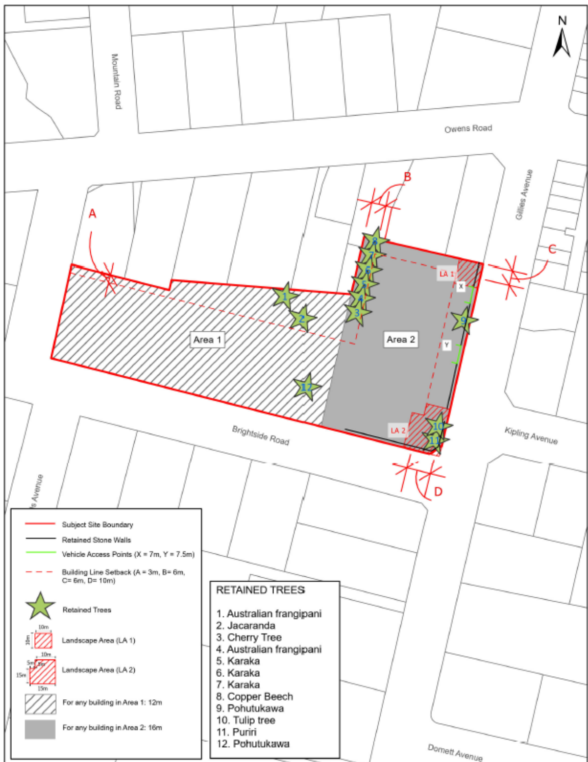
Figure H25.6.1.2 Brightside Hospital Plan
