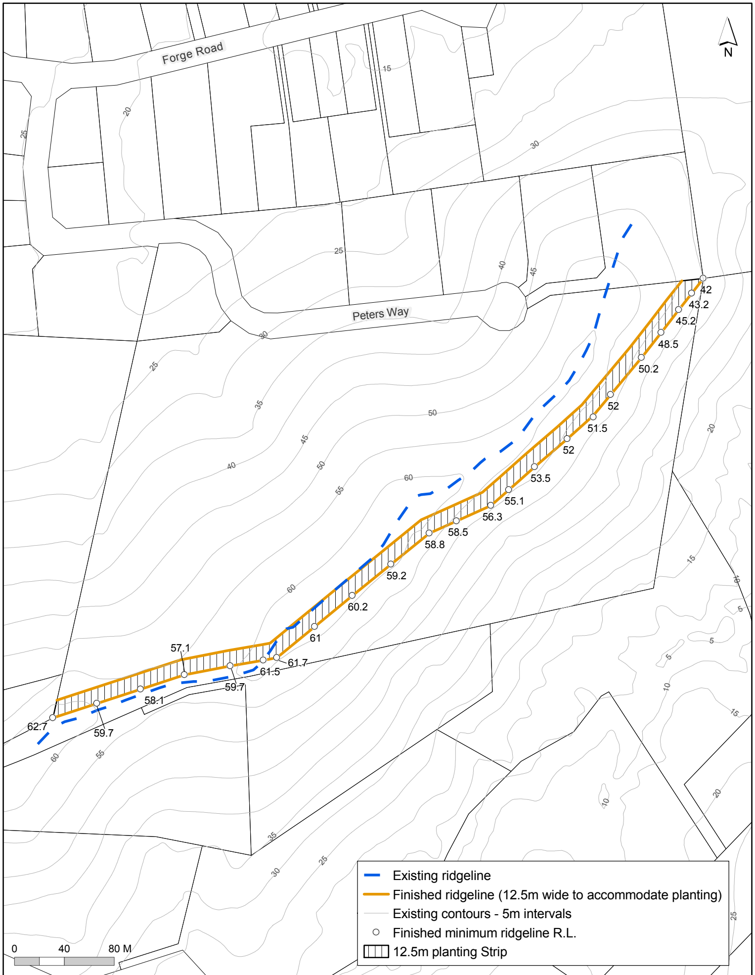
Silverdale 1: Ridgeline finished relative levels (RL)
