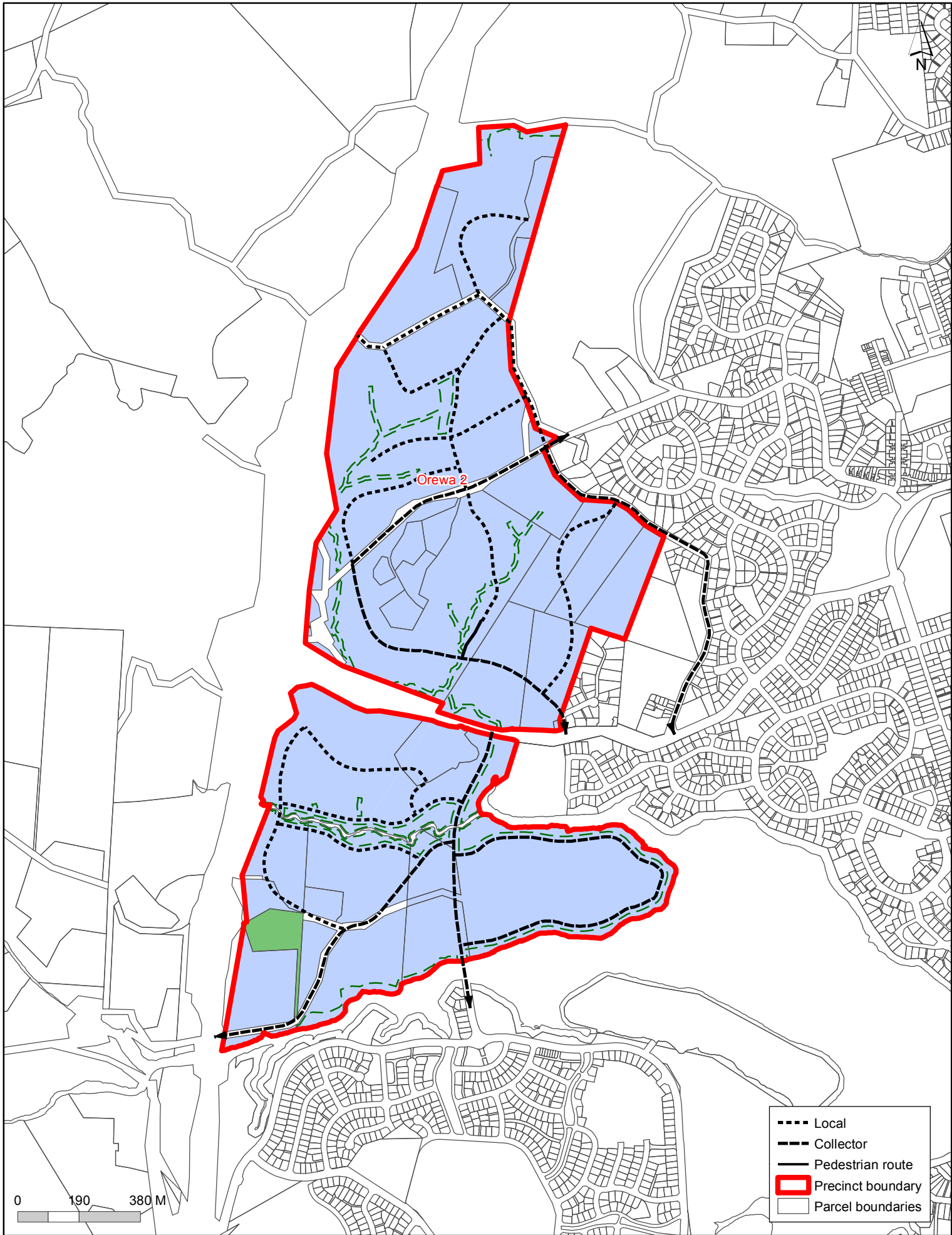
Orewa 2 Precinct Plan 3: Road hierarchy
