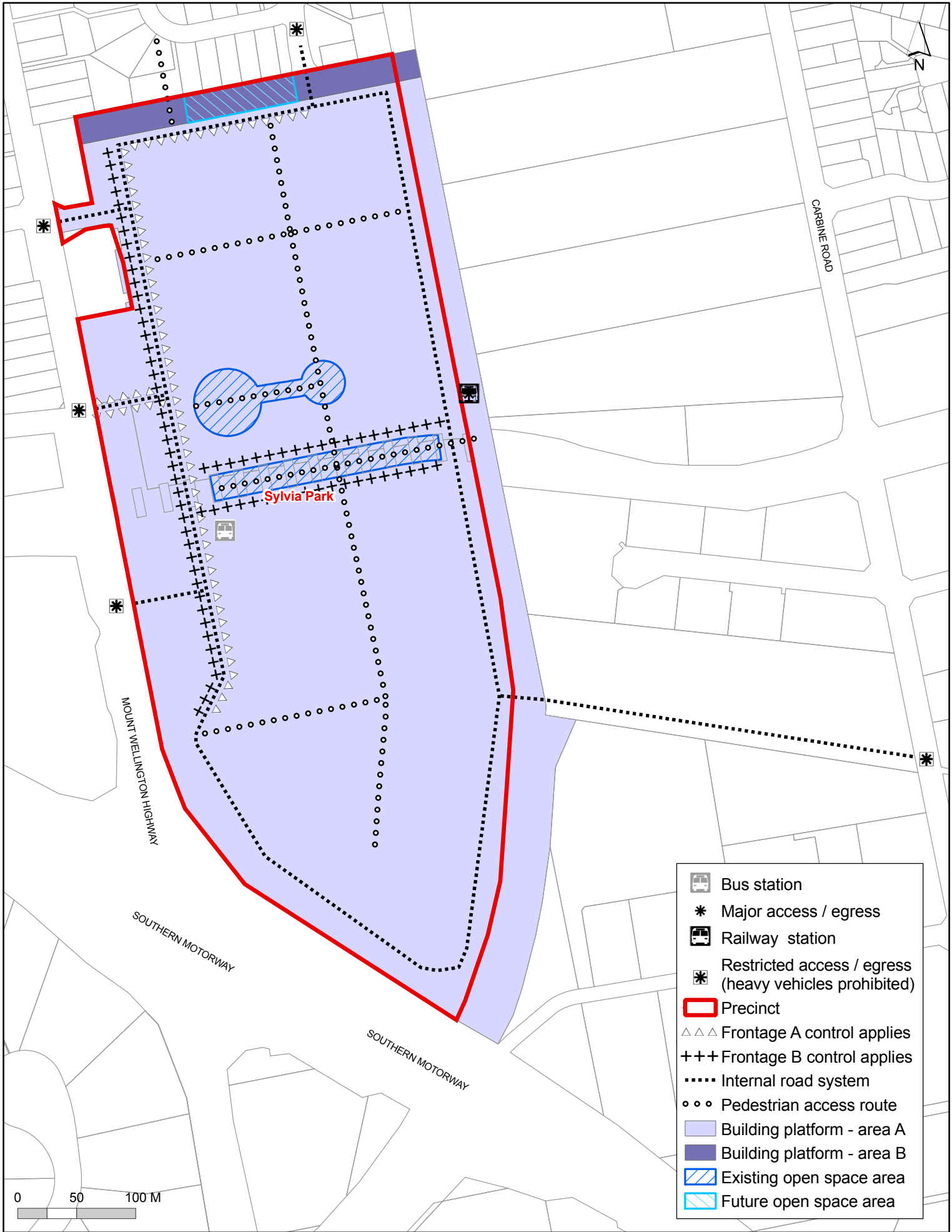
Sylvia Park Precinct Plan 2 – Structural Elements
