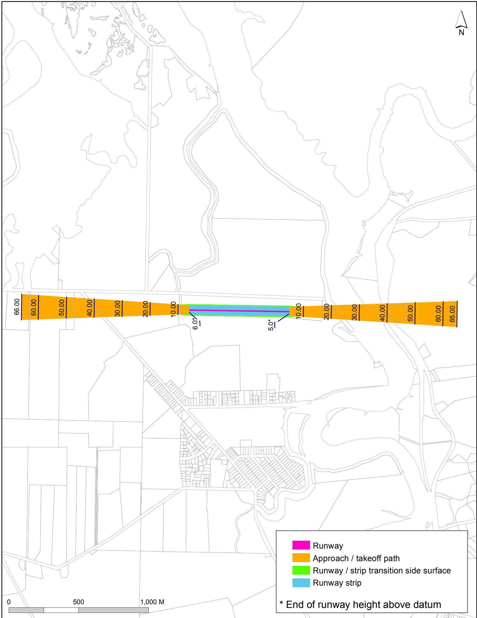
Airport approach path: Parakai Airfield height restriction
