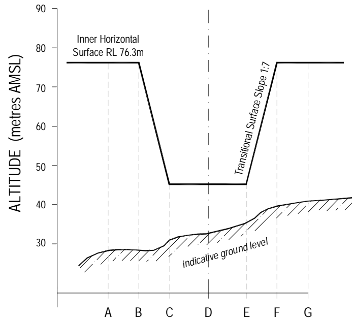
TYPICAL CROSS SECTION A - G
