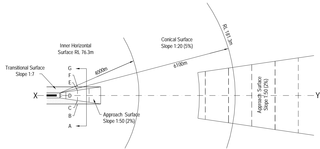
TYPICAL PLAN VIEW
