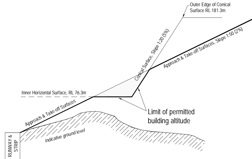
TYPICAL LONG SECTION X - Y
