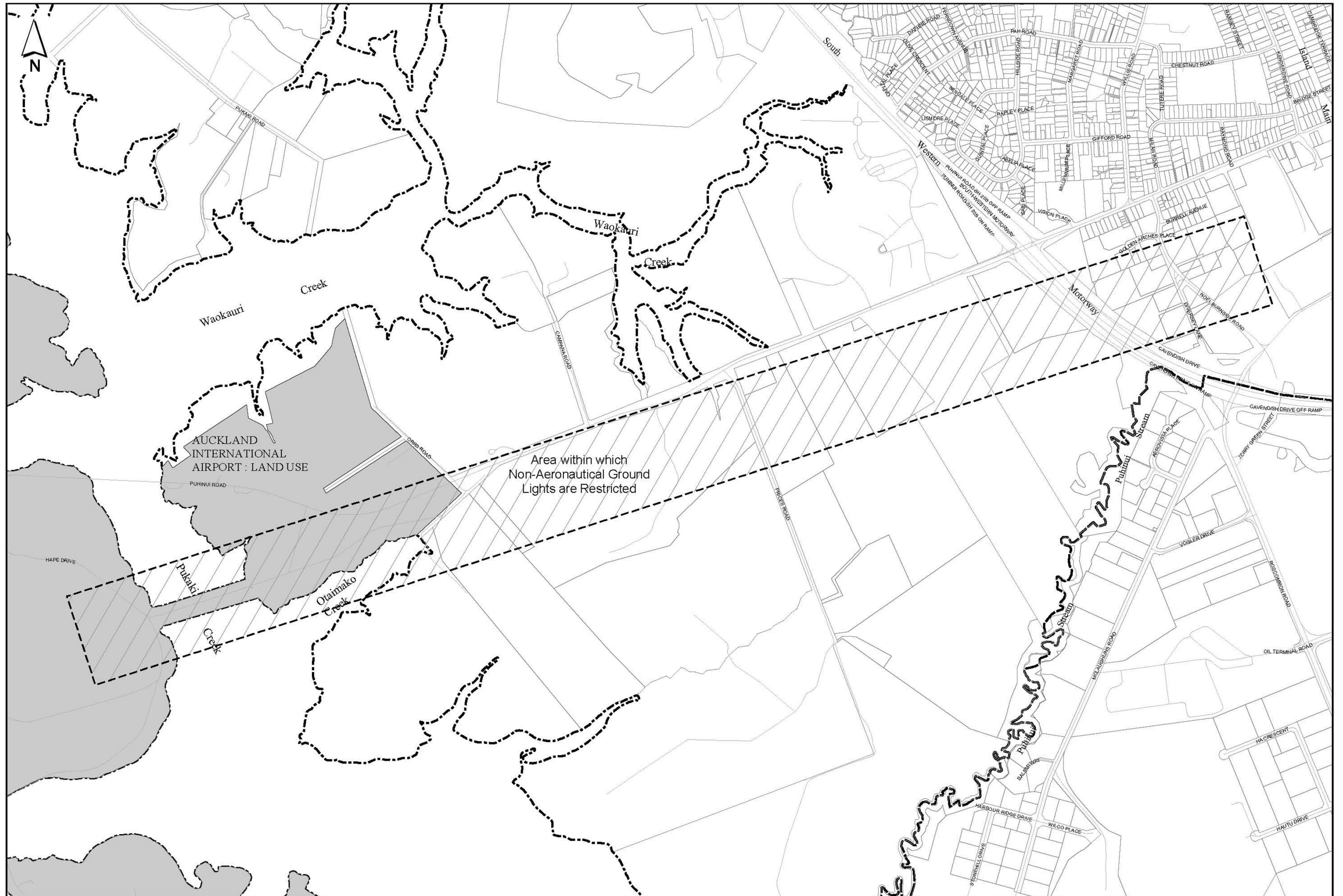
Figure 4 - REQUIREMENTS FOR NON-AERONAUTICAL GROUND LIGHTS APPENDIX 3
