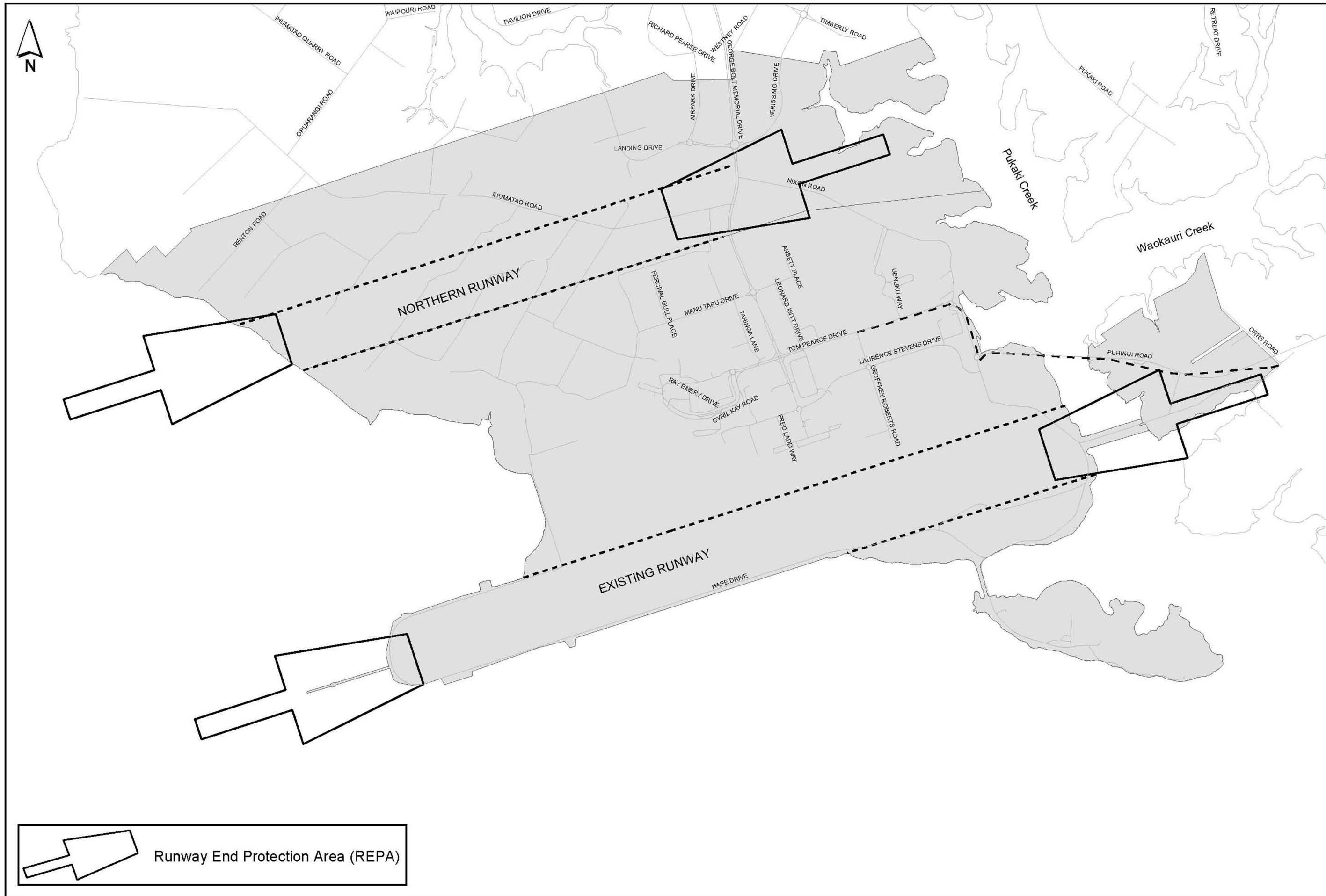
Figure 3 - RUNWAY END PROTECTION AREAS APPENDIX 2
