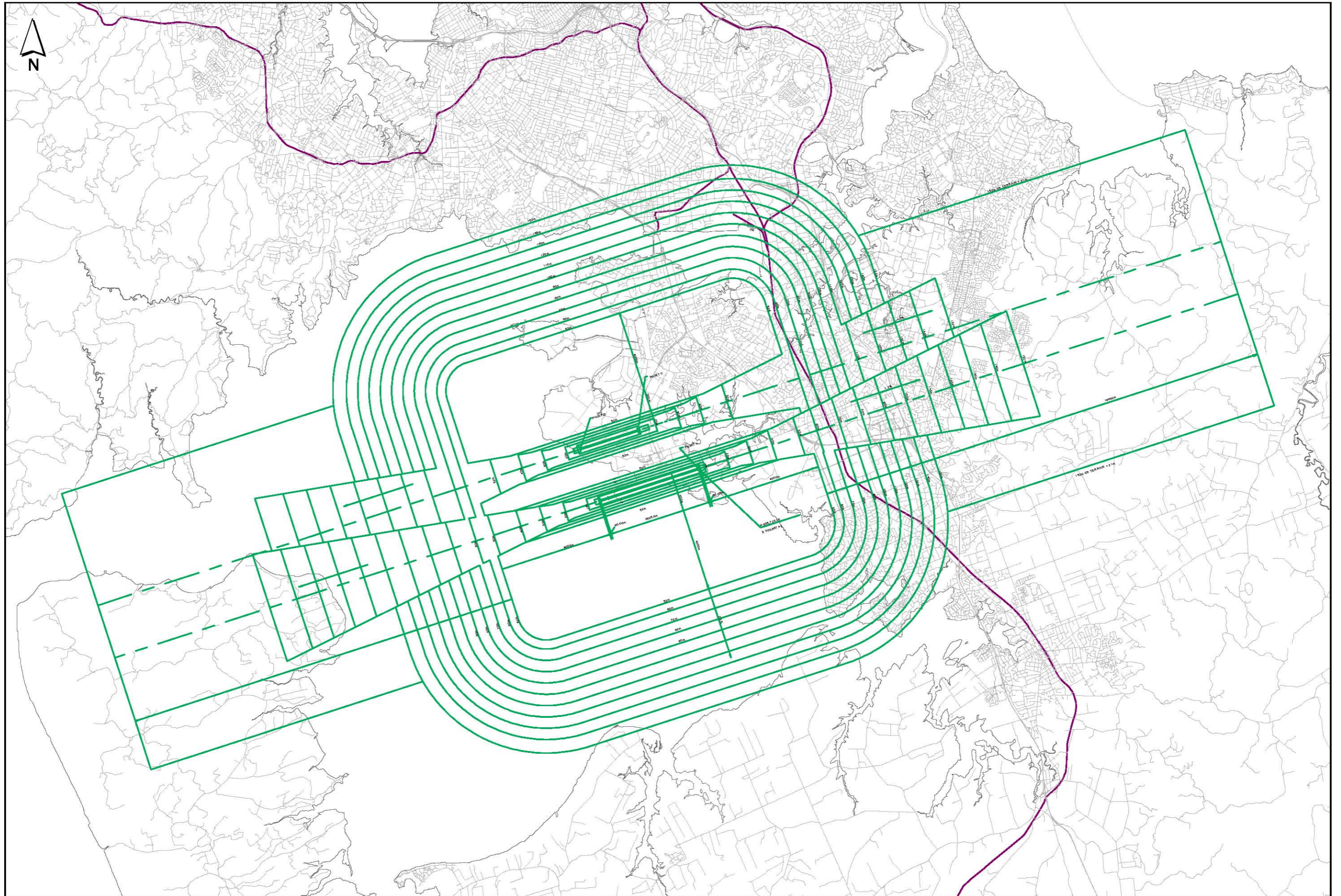
Figure 1 - SPECIFICATION FOR OBSTACLE LIMITATION SURFACES
